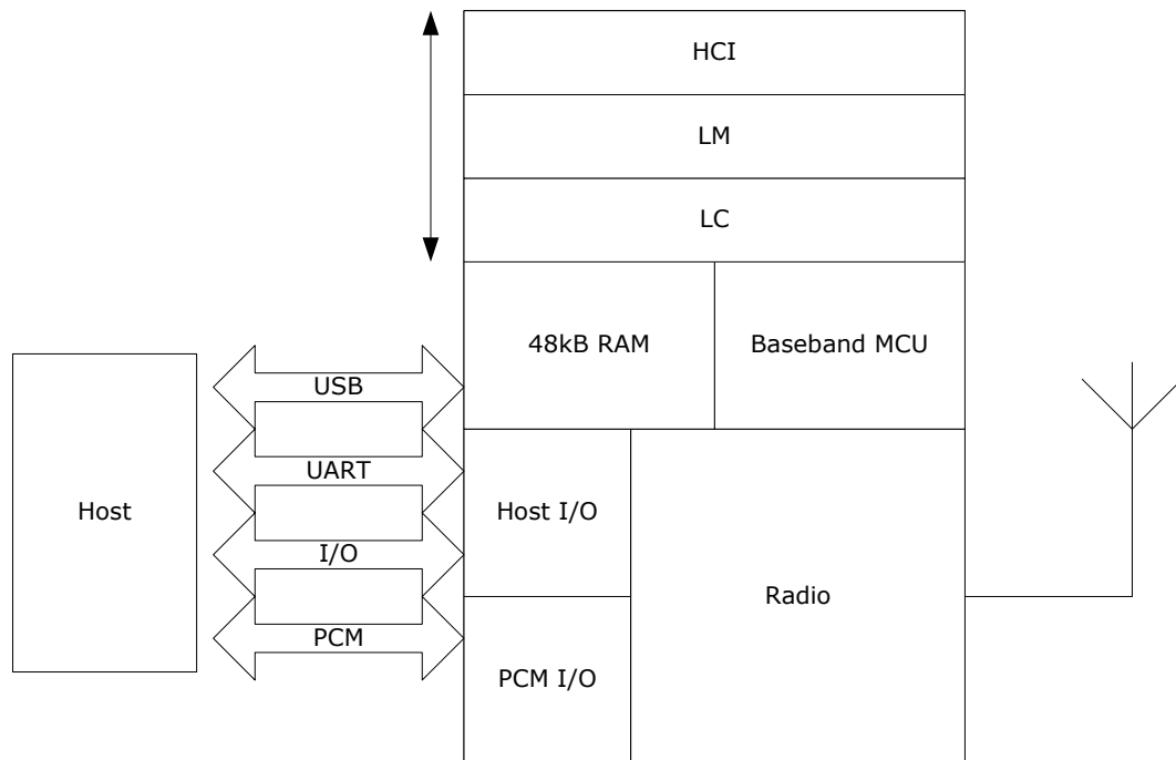
Figure 23: HCI Stack
